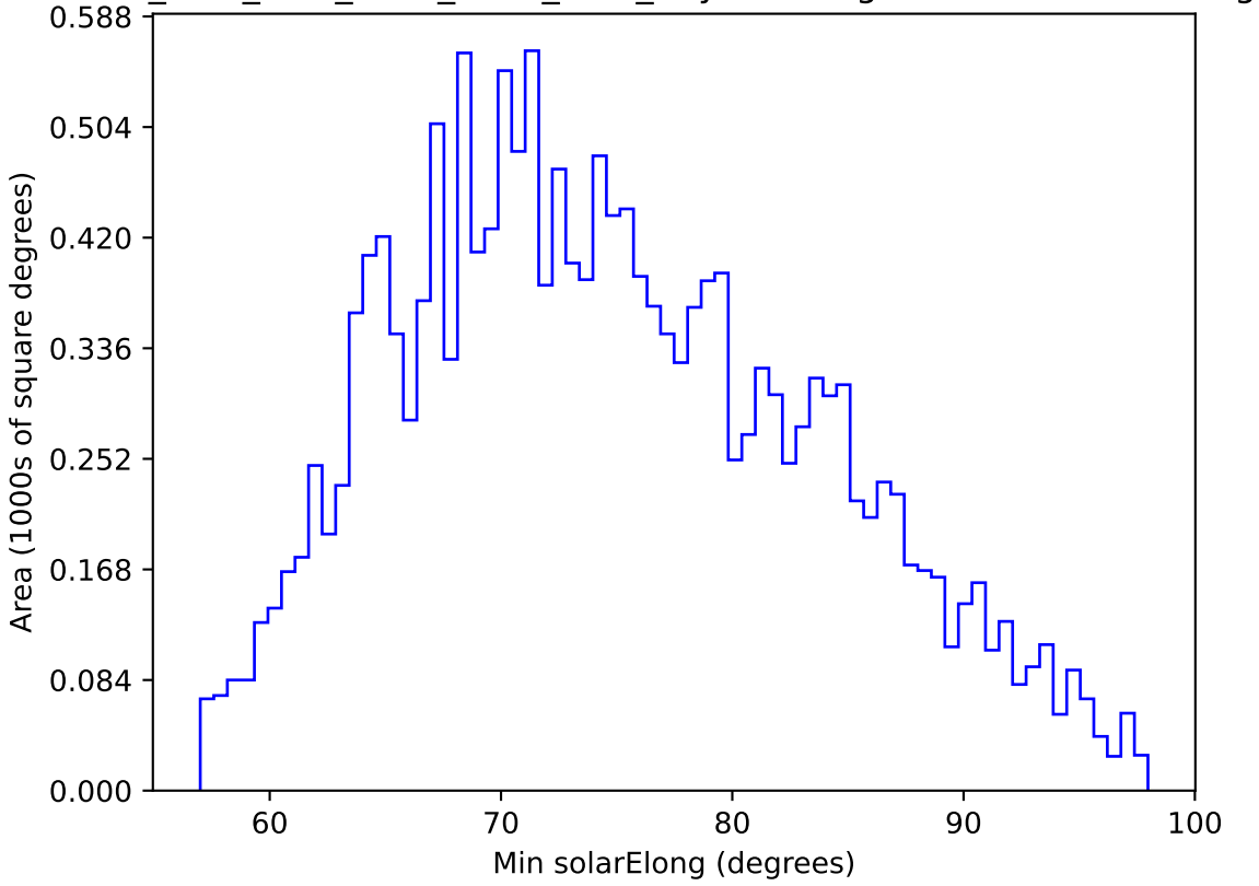
ddf_acor_sf25_lsf40_lsr10_v3.4_10yrs WFD g band: Min solarElong
