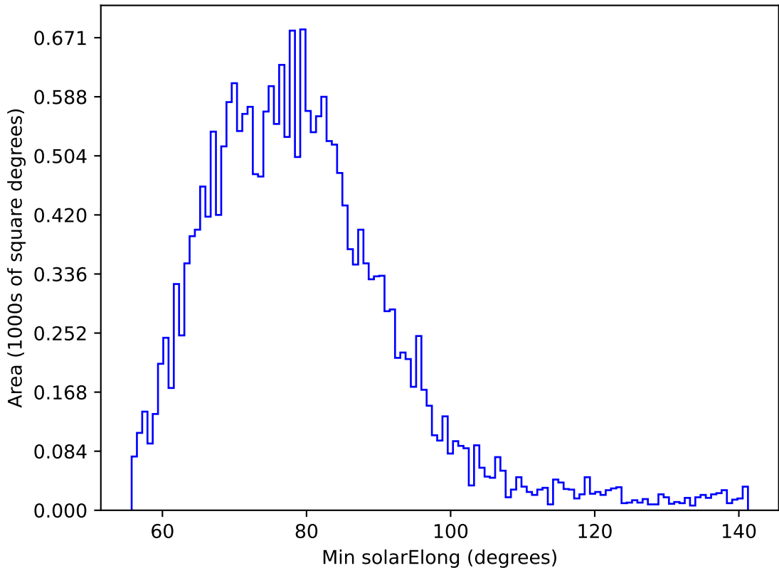
ddf_acor_sf25_lsf40_lsr10_v3.4_10yrs All sky u band: Min solarElong
