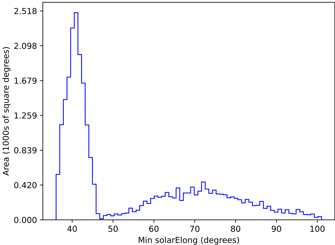
ddf_acor_sf25_lsf40_lsr10_v3.4_10yrs All sky i band: Min solarElong
