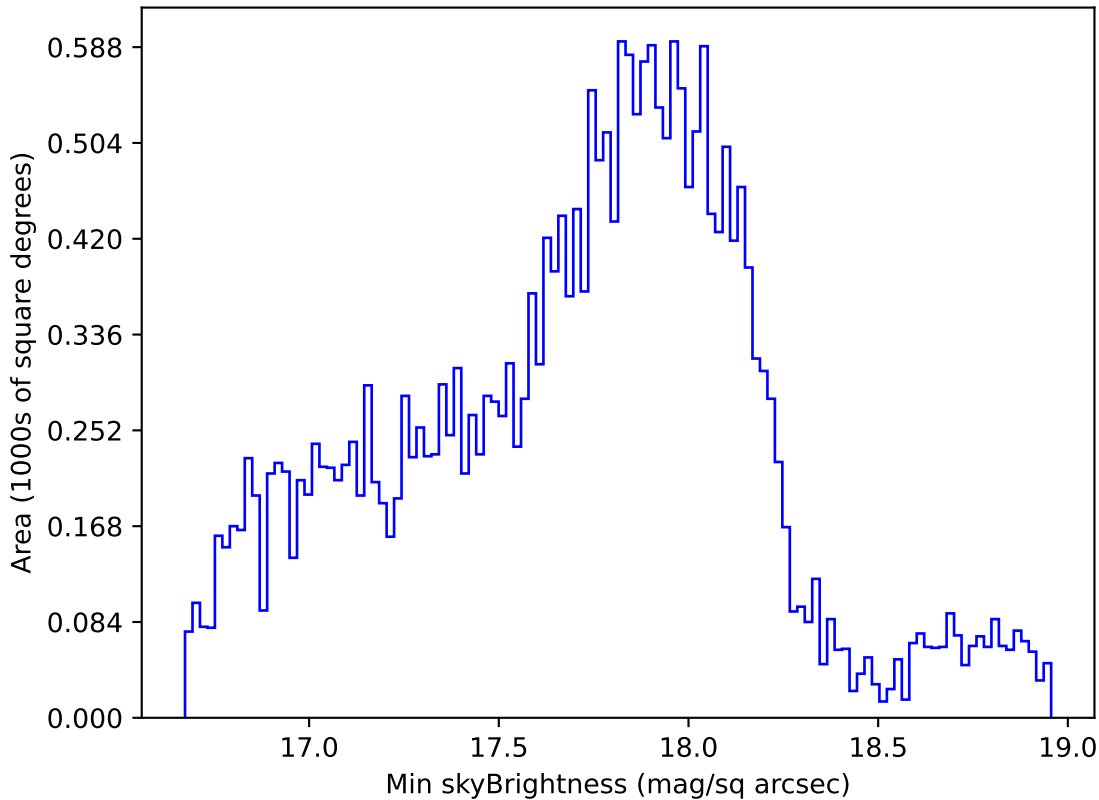
ddf_acor_sf25_lsf40_lsr10_v3.4_10yrs Yr 1 all bands: Min skyBrightness
