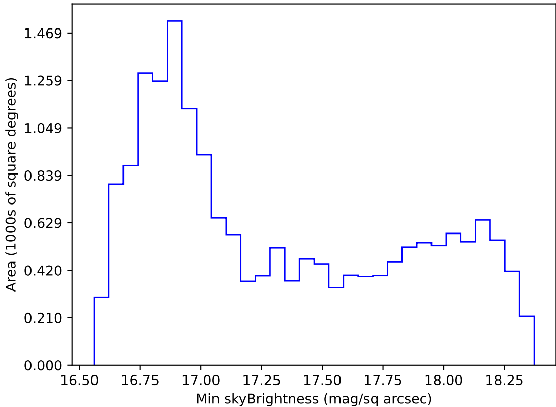
ddf_acor_sf25_lsf40_lsr10_v3.4_10yrs WFD z band: Min skyBrightness
