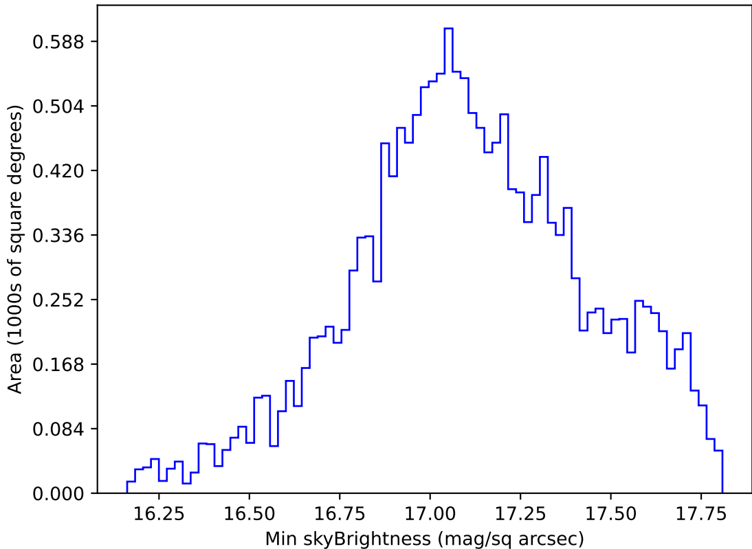
ddf_acor_sf25_lsf40_lsr10_v3.4_10yrs WFD y band: Min skyBrightness
