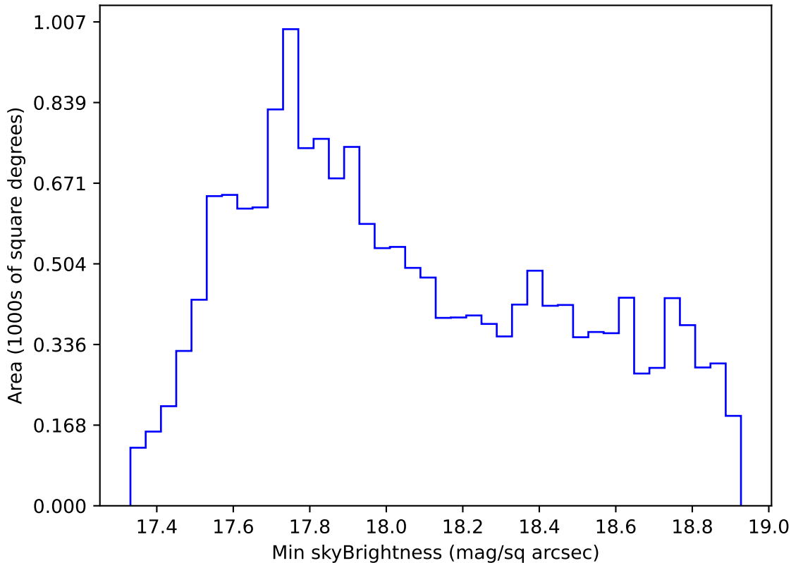
ddf_acor_sf25_lsf40_lsr10_v3.4_10yrs WFD i band: Min skyBrightness
