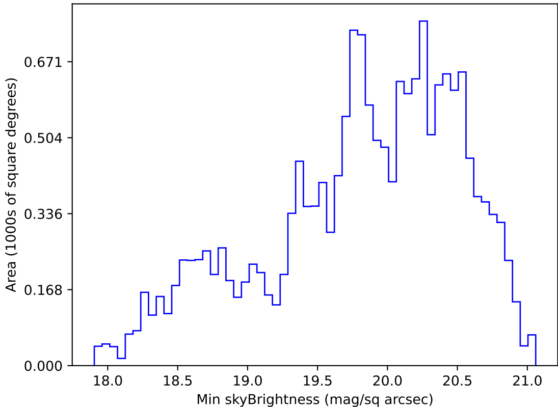
ddf_acor_sf25_lsf40_lsr10_v3.4_10yrs WFD g band: Min skyBrightness
