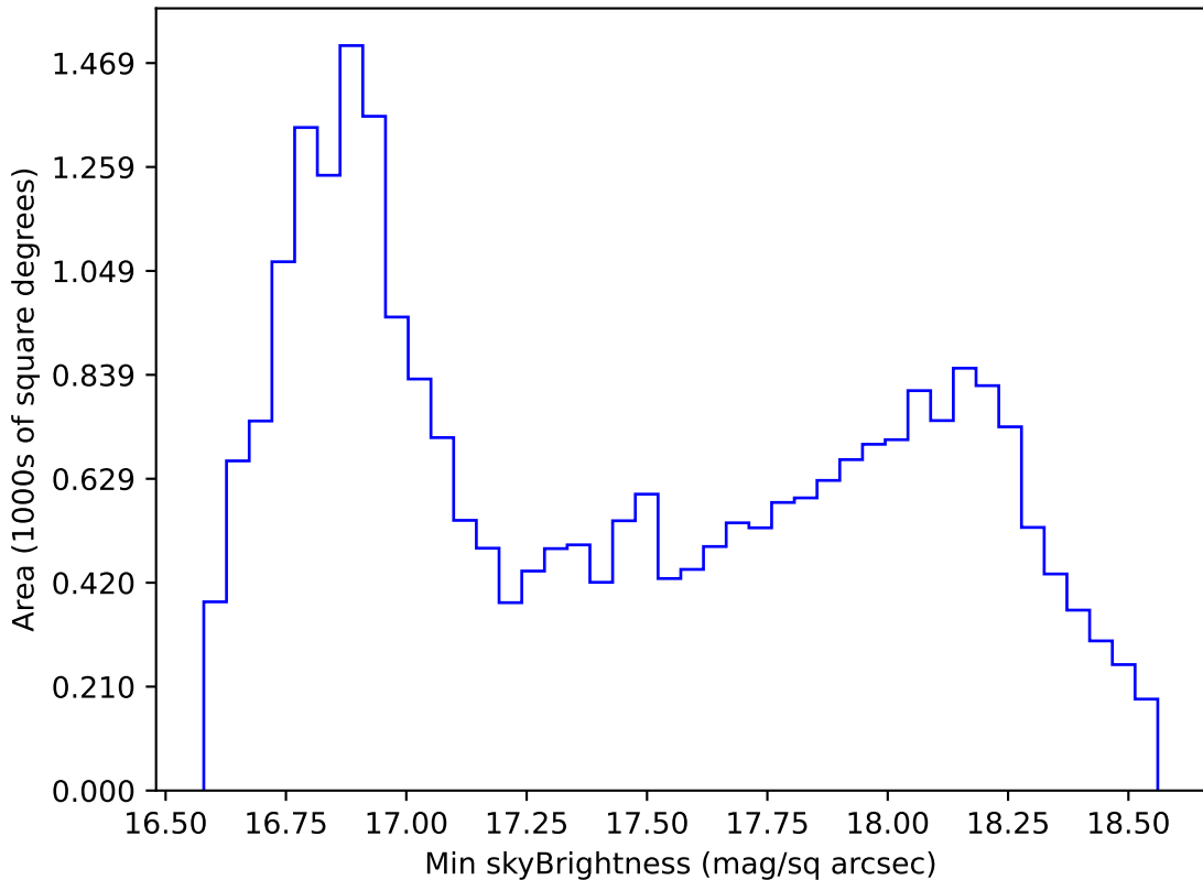
ddf_acor_sf25_lsf40_lsr10_v3.4_10yrs All sky z band: Min skyBrightness
