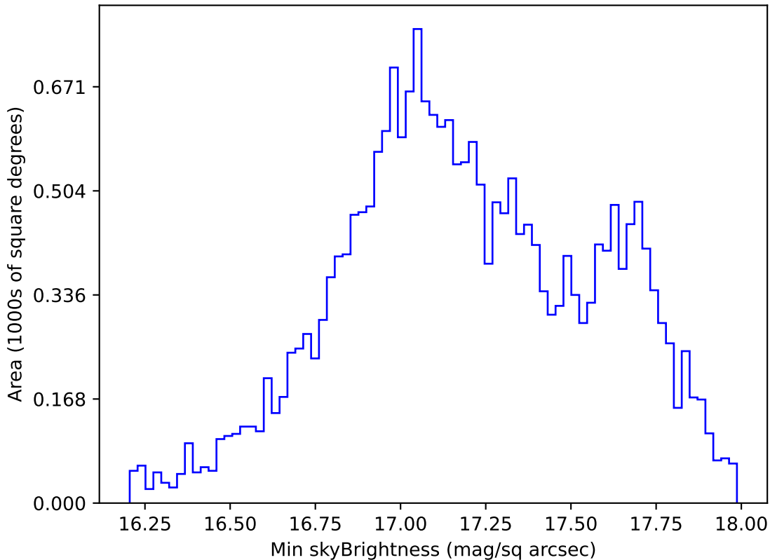
ddf_acor_sf25_lsf40_lsr10_v3.4_10yrs All sky y band: Min skyBrightness
