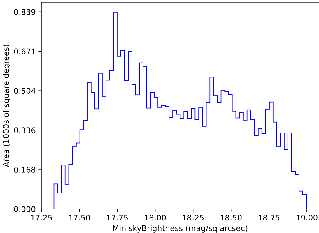
ddf_acor_sf25_lsf40_lsr10_v3.4_10yrs All sky i band: Min skyBrightness
