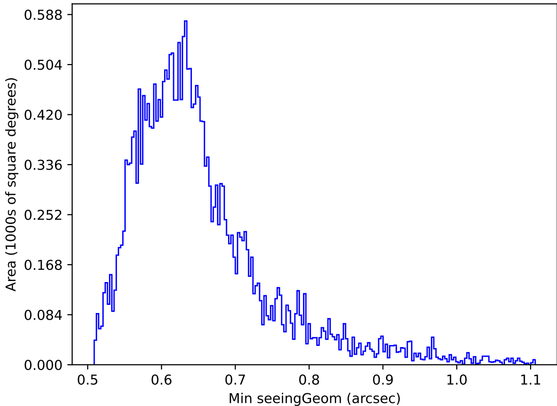
ddf_acor_sf25_lsf40_lsr10_v3.4_10yrs Yr 1 z band: Min seeingGeom
