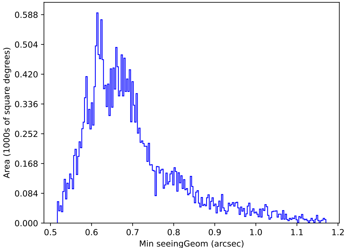
ddf_acor_sf25_ls40_lsr10_v3.4_10yrs Yr 1 g band: Min seeingGeom
