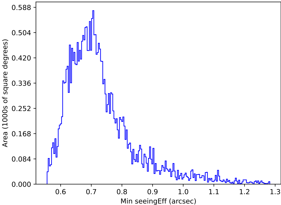
ddf_acor_sf25_lsf40_lsr10_v3.4_10yrs Yr 1 z band: Min seeingEff
