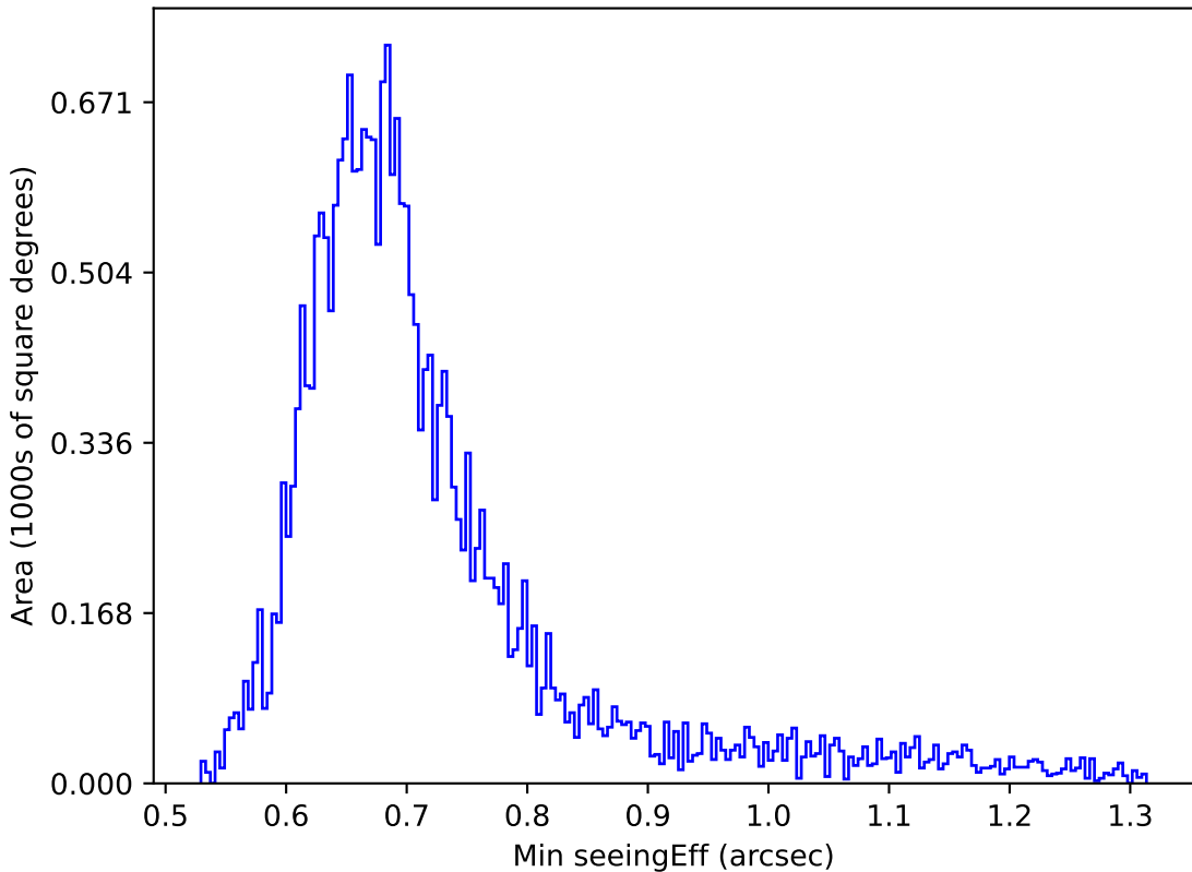
ddf_acor_sf25_lsf40_lsr10_v3.4_10yrs Yr 1 r band: Min seeingEff
