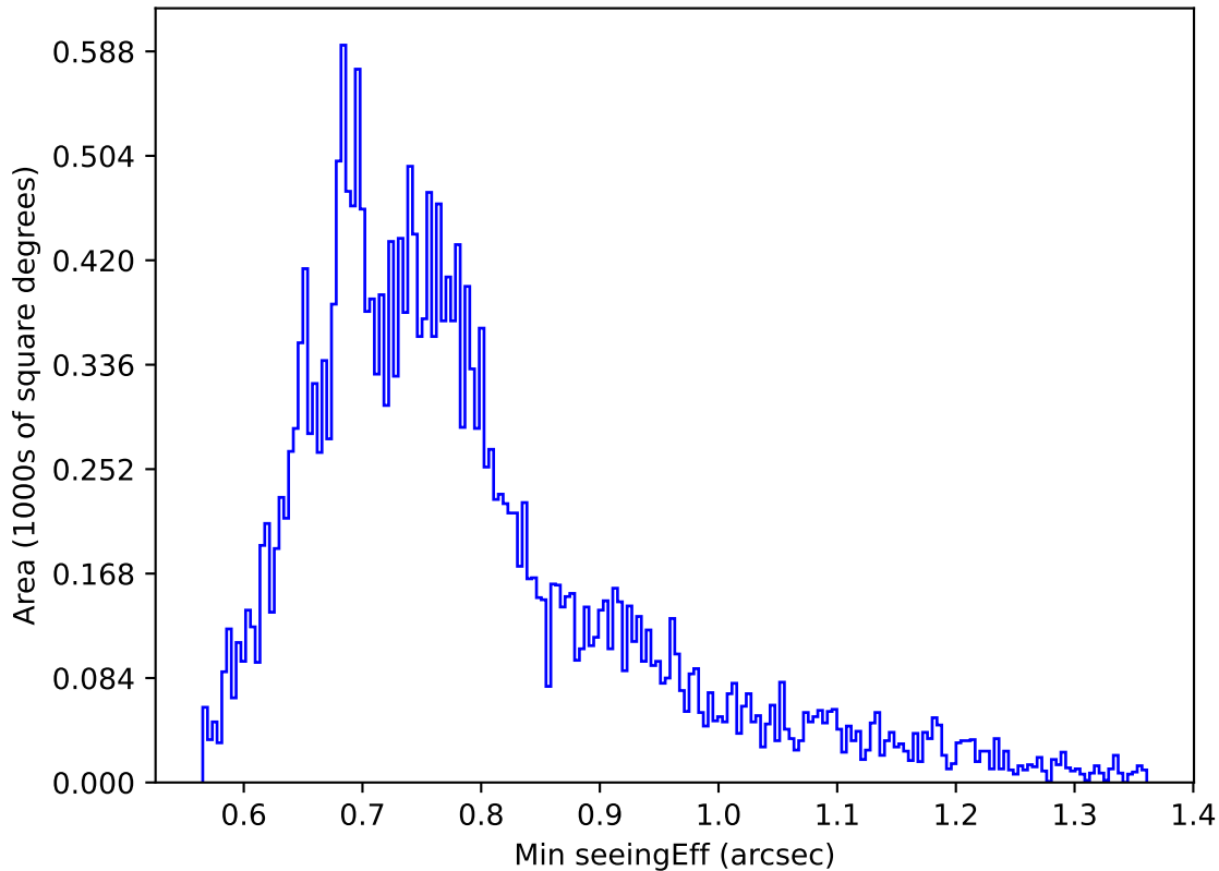
ddf_acor_sf25_lsf40_lsr10_v3.4_10yrs Yr 1 g band: Min seeingEff
