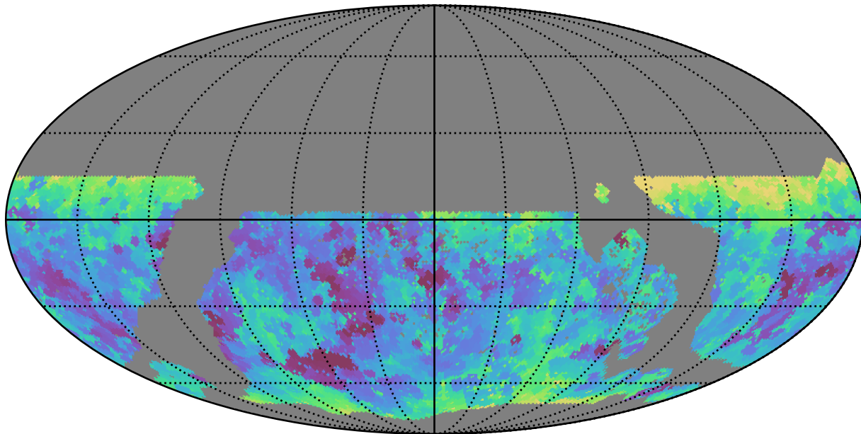
ddf_acor_sf25_lsf40_lsr10_v3.4_10yrs WFD r band: Min seeingEff
