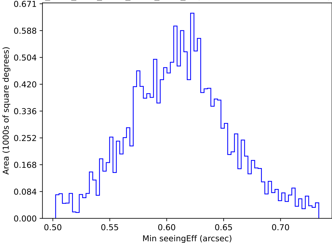
ddf_acor_sf25_lsf40_lsr10_v3.4_10yrs WFD r band: Min seeingEff
