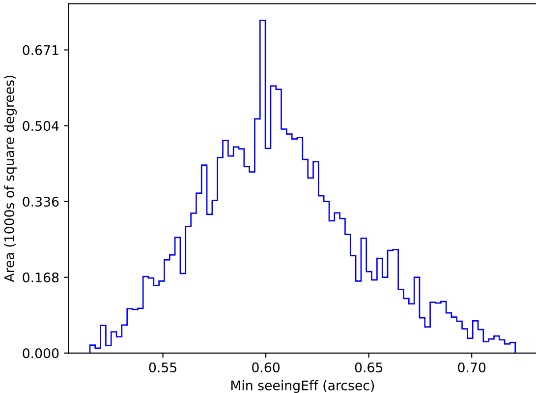
ddf_acor_sf25_lsf40_lsr10_v3.4_10yrs WFD i band: Min seeingEff
