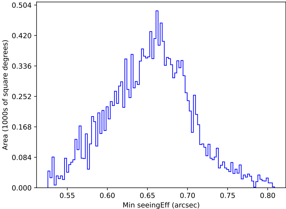
ddf_acor_sf25_lsf40_lsr10_v3.4_10yrs WFD g band: Min seeingEff
