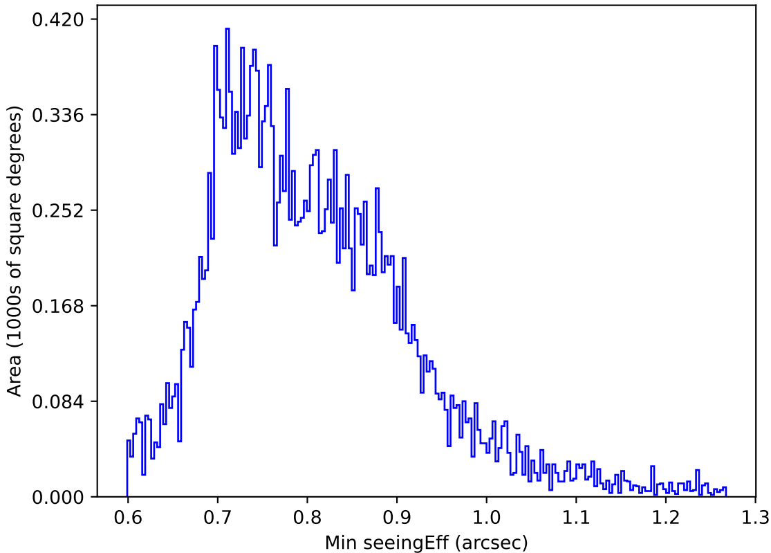
ddf_acor_sf25_lsf40_lsr10_v3.4_10yrs All sky u band: Min seeingEff
