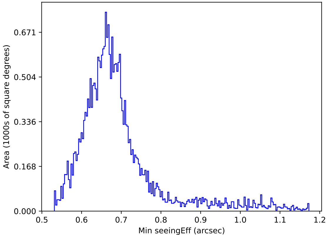
ddf_acor_sf25_lsf40_lsr10_v3.4_10yrs All sky g band: Min seeingEff
