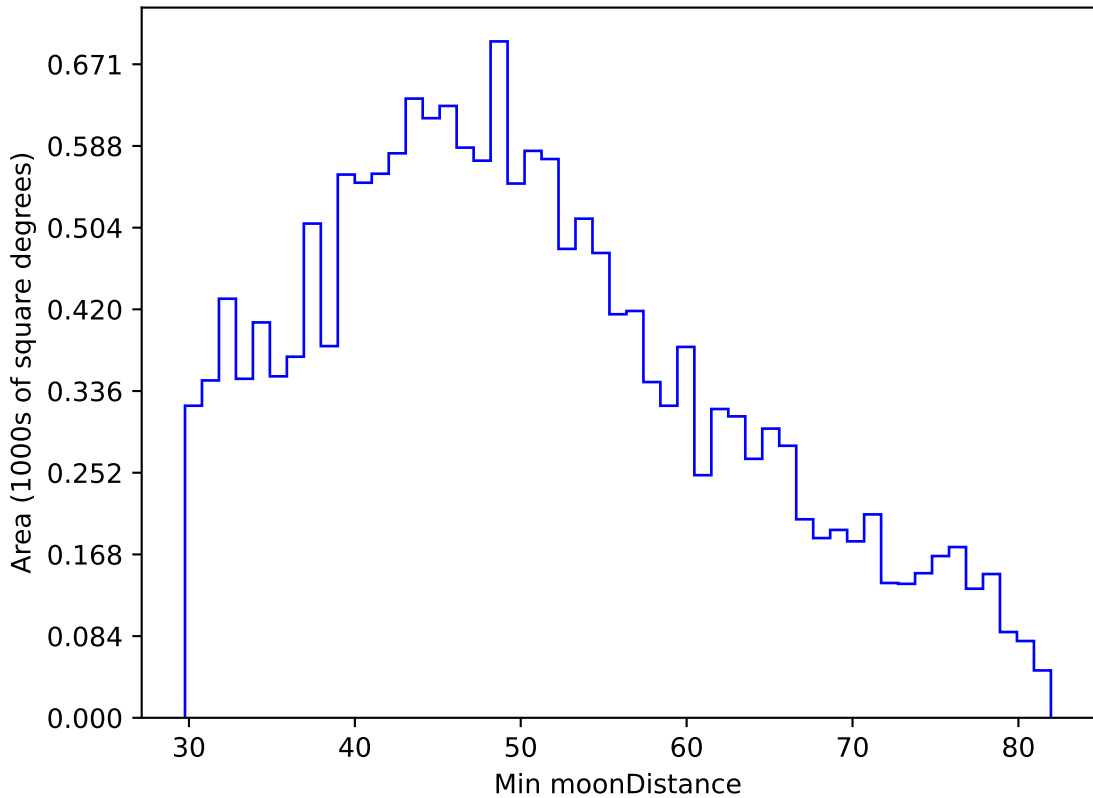
ddf_acor_sf25_lsf40_lsr10_v3.4_10yrs WFD u band: Min moonDistance
