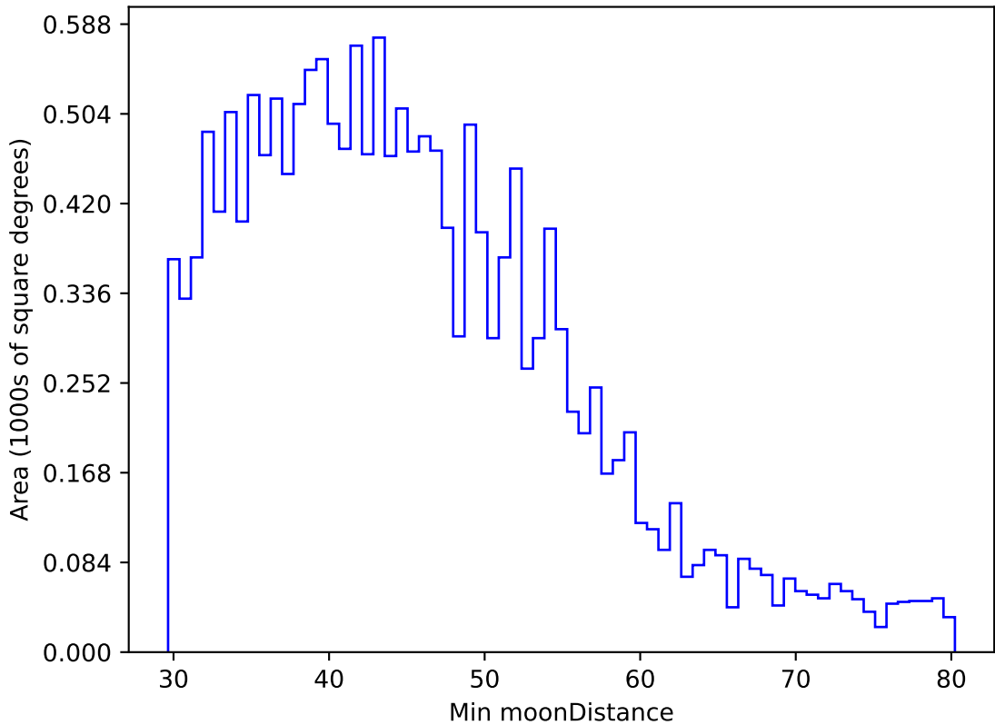
ddf_acor_sf25_lsf40_lsr10_v3.4_10yrs WFD g band: Min moonDistance
