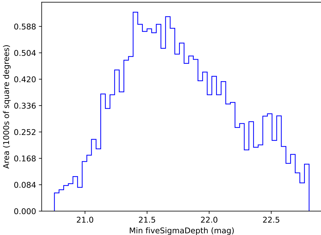
ddf_acor_sf25_ls40_lsr10_v3.4_10yrs WFD i band: Min fiveSigmaDepth
