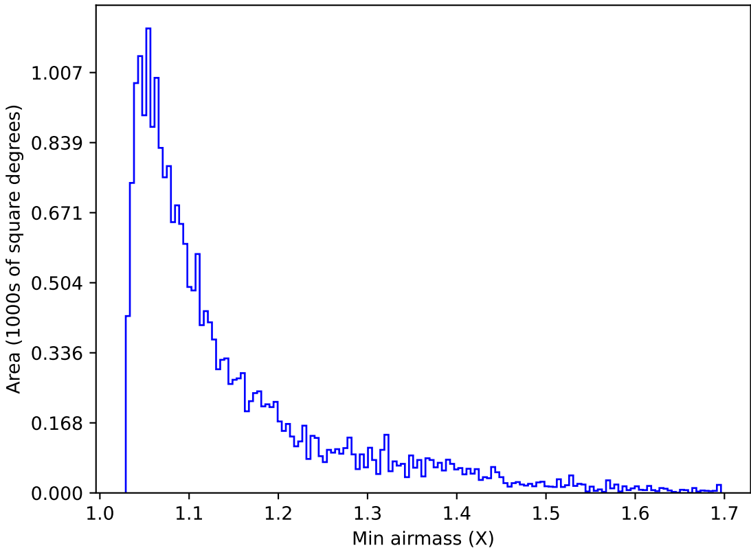
ddf_acor_sf25_lsf40_lsr10_v3.4_10yrs Yr 1 u band: Min airmass
