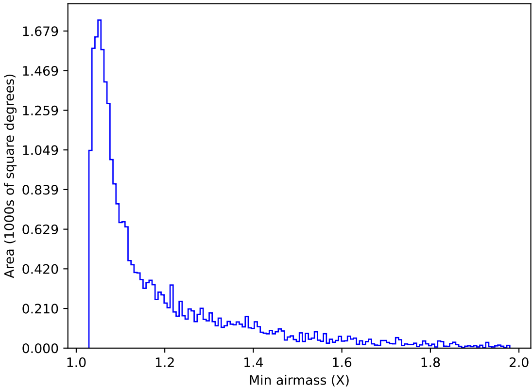
ddf_acor_sf25_lsf40_lsr10_v3.4_10yrs Yr 1 g band: Min airmass
