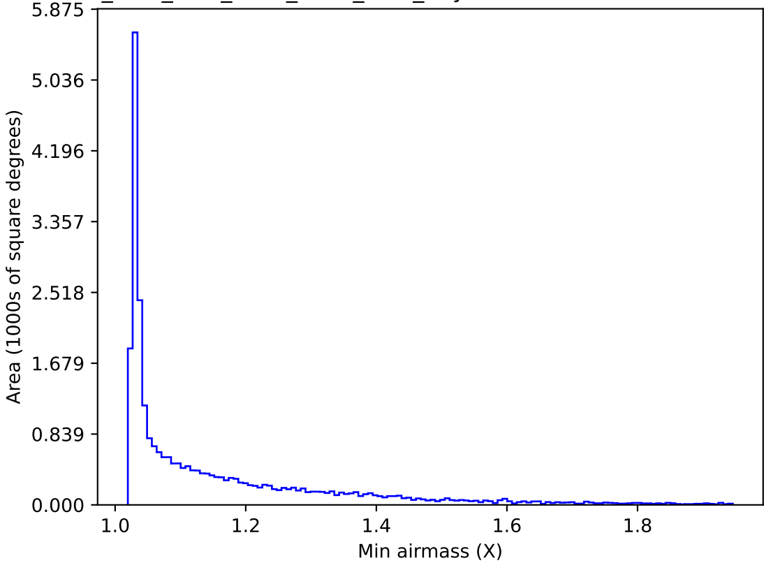
ddf_acor_sf25_lsf40_lsr10_v3.4_10yrs Yr 1 all bands: Min airmass
