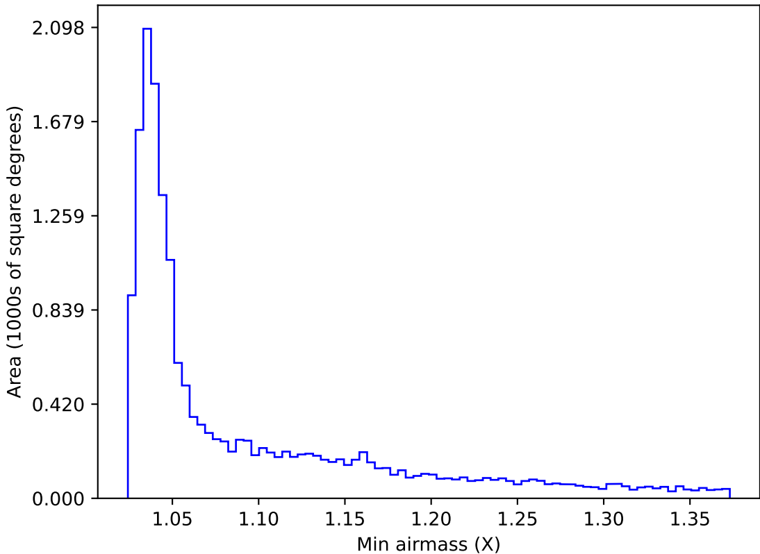
ddf_acor_sf25_lsf40_lsr10_v3.4_10yrs WFD u band: Min airmass
