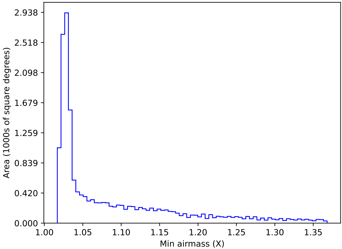
ddf_acor_sf25_lsf40_lsr10_v3.4_10yrs WFD r band: Min airmass
