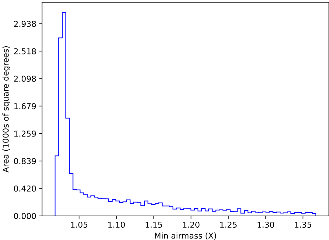
ddf_acor_sf25_lsf40_lsr10_v3.4_10yrs WFD i band: Min airmass
