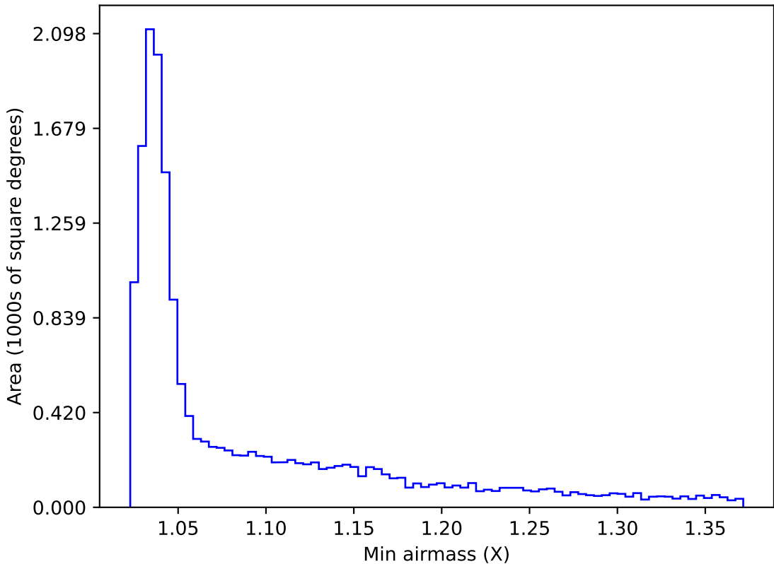
ddf_acor_sf25_lsf40_lsr10_v3.4_10yrs WFD g band: Min airmass
