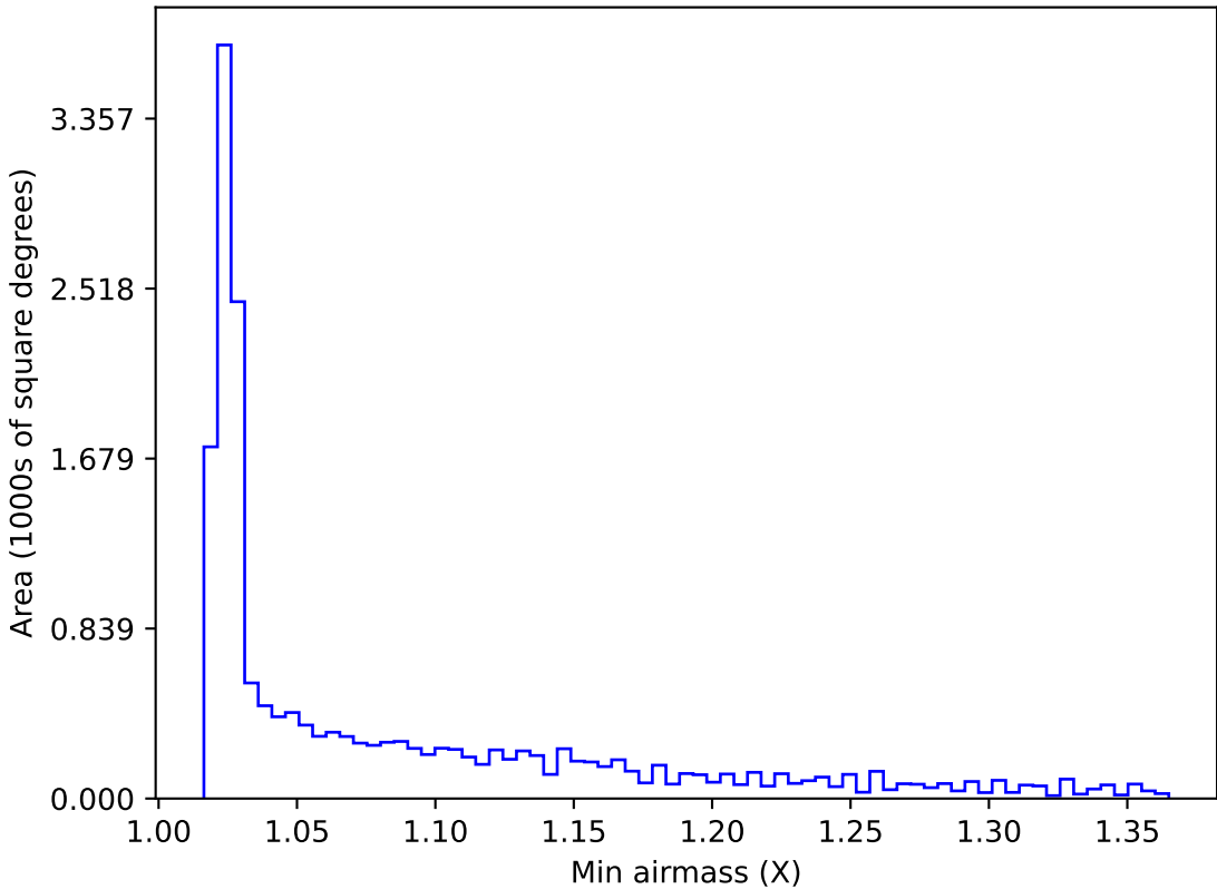
ddf_acor_sf25_lsf40_lsr10_v3.4_10yrs WFD all bands: Min airmass
