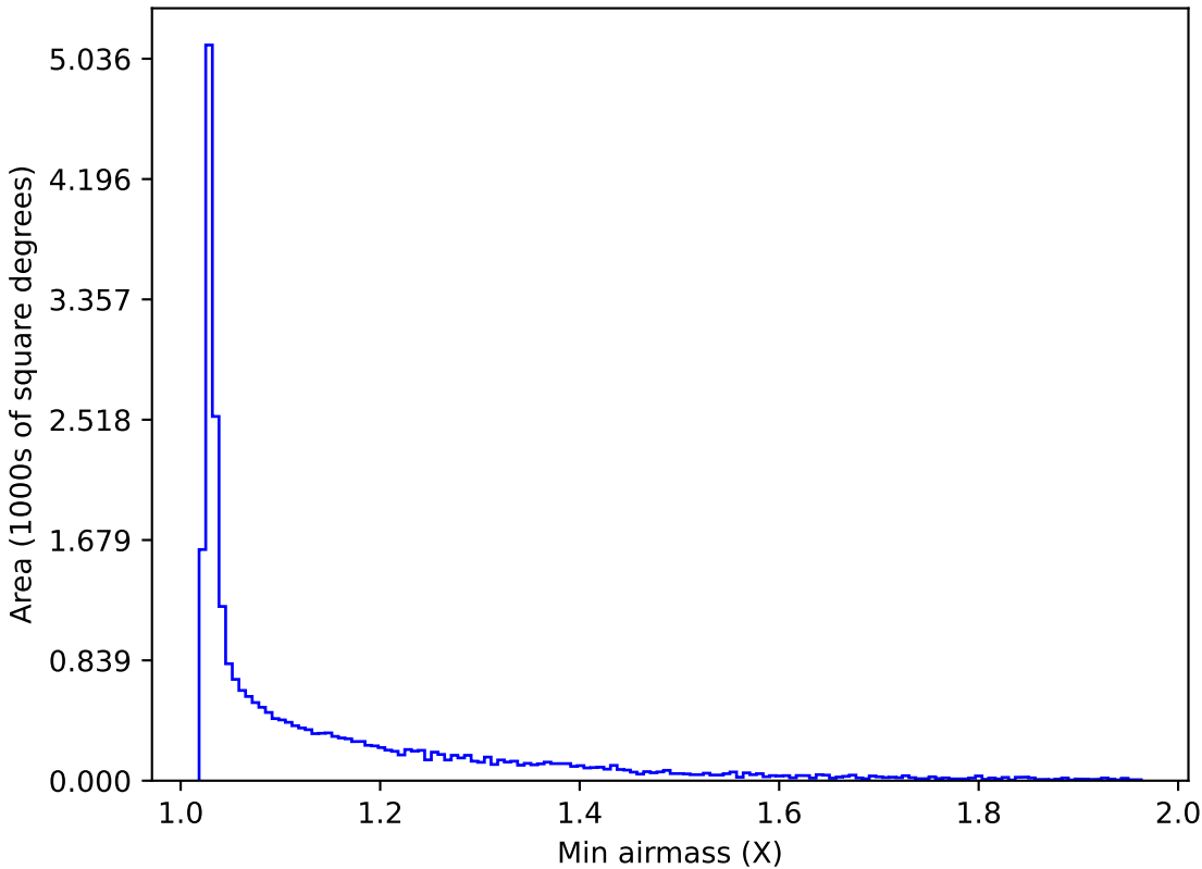
ddf_acor_sf25_lsf40_lsr10_v3.4_10yrs All sky z band: Min airmass
