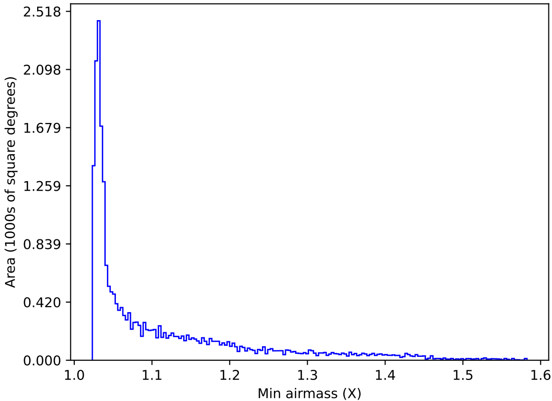
ddf_acor_sf25_lsf40_lsr10_v3.4_10yrs All sky y band: Min airmass
