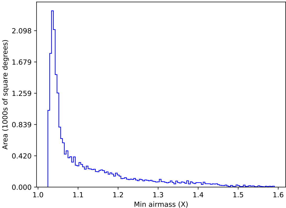
ddf_acor_sf25_lsf40_lsr10_v3.4_10yrs All sky u band: Min airmass
