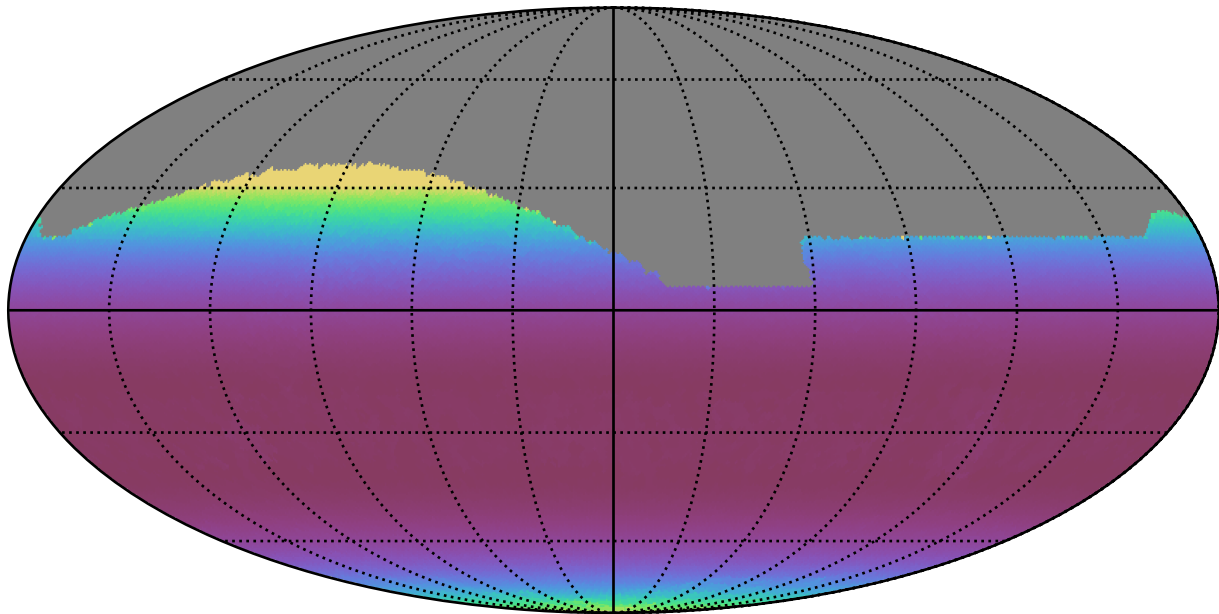
ddf_acor_sf25_lsf40_lsr10_v3.4_10yrs All sky r band: Min airmass
