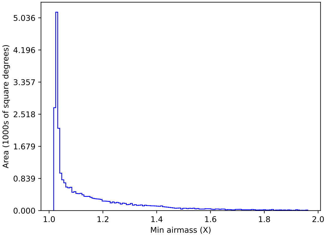
ddf_acor_sf25_lsf40_lsr10_v3.4_10yrs All sky r band: Min airmass
