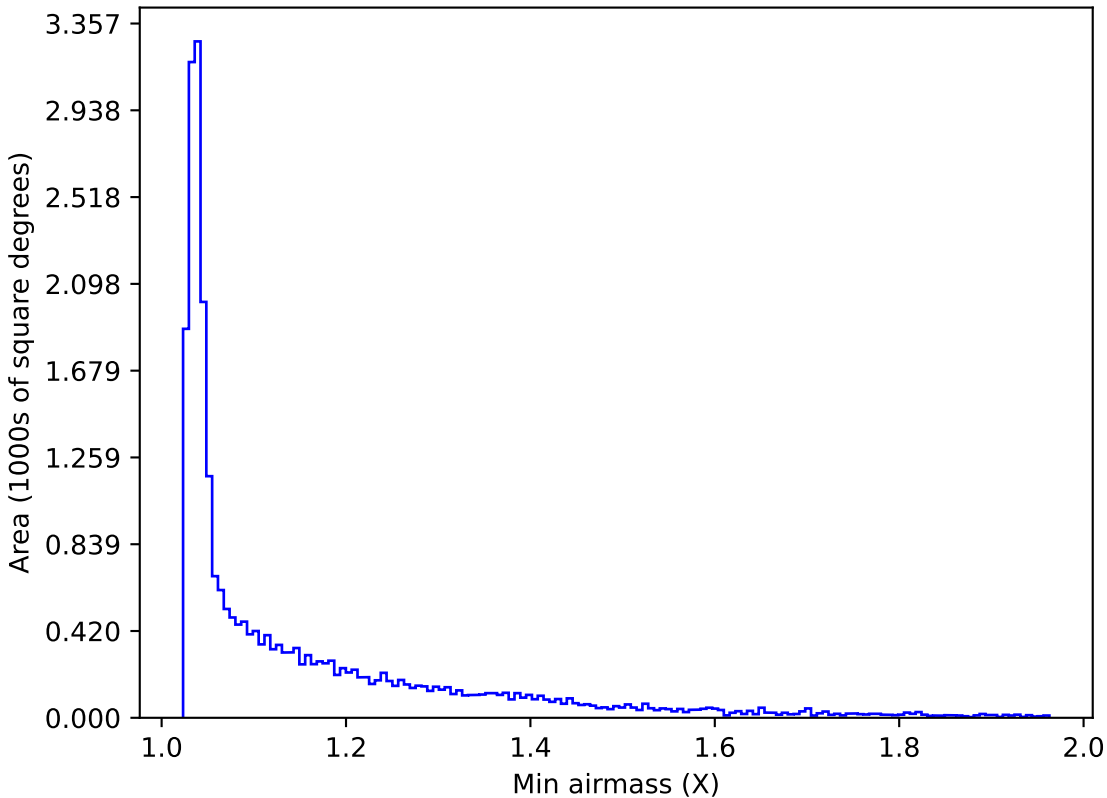
ddf_acor_sf25_lsf40_lsr10_v3.4_10yrs All sky g band: Min airmass
