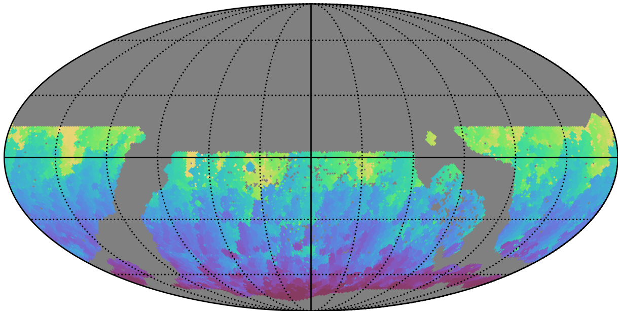
ddf_acor_sf25_lsf40_lsr10_v3.4_10yrs WFD g band: Min HA
