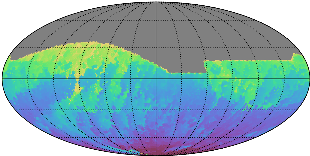
ddf_acor_sf25_lsf40_lsr10_v3.4_10yrs All sky z band: Min HA
