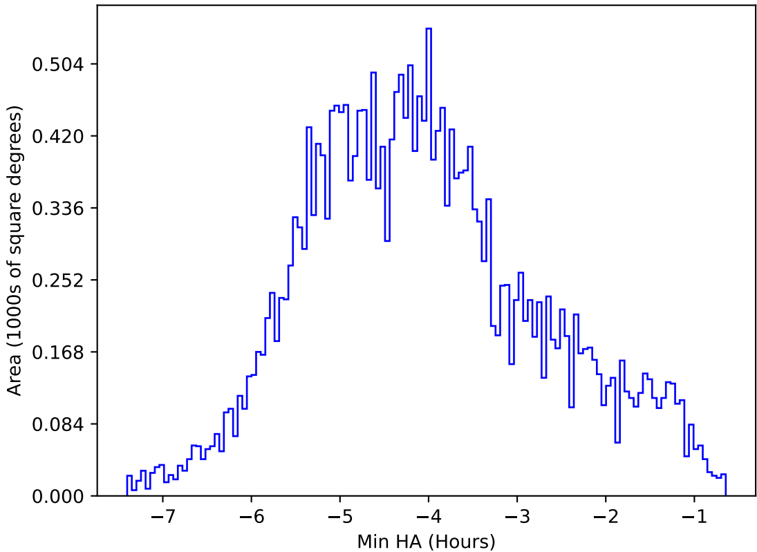
ddf_acor_sf25_lsf40_lsr10_v3.4_10yrs All sky z band: Min HA
