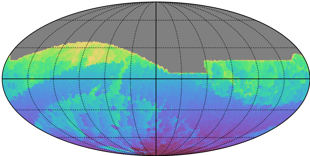
ddf_acor_sf25_lsf40_lsr10_v3.4_10yrs All sky r band: Min HA
