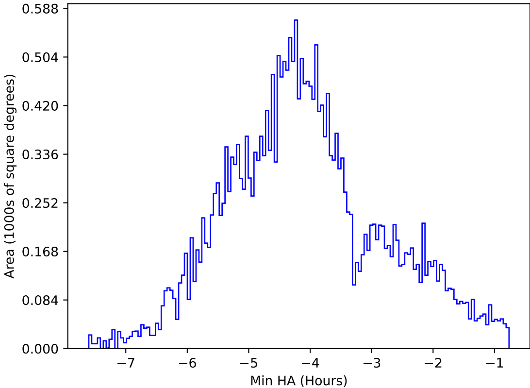
ddf_acor_sf25_lsf40_lsr10_v3.4_10yrs All sky i band: Min HA
