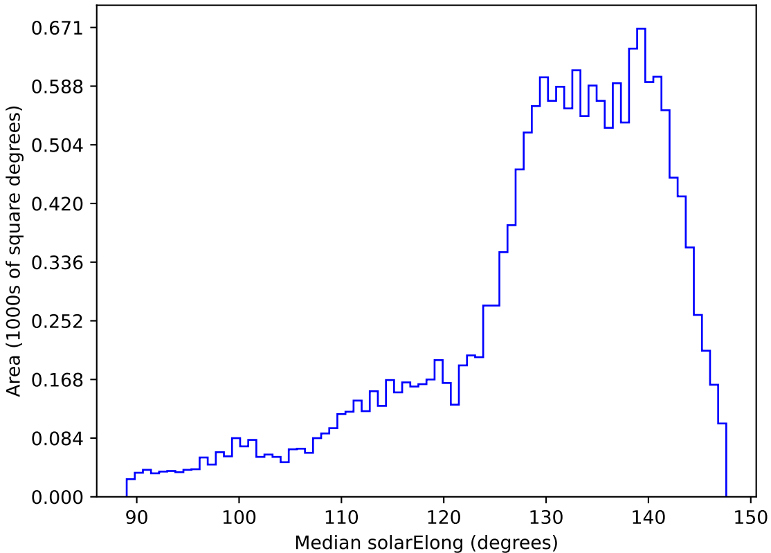
ddf_acor_sf25_lsf40_lsr10_v3.4_10yrs WFD y band: Median solarElong
