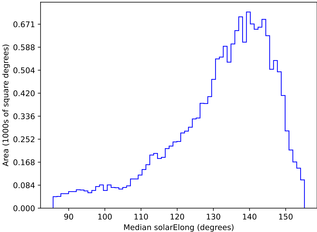
ddf_acor_sf25_lsf40_lsr10_v3.4_10yrs WFD u band: Median solarElong
