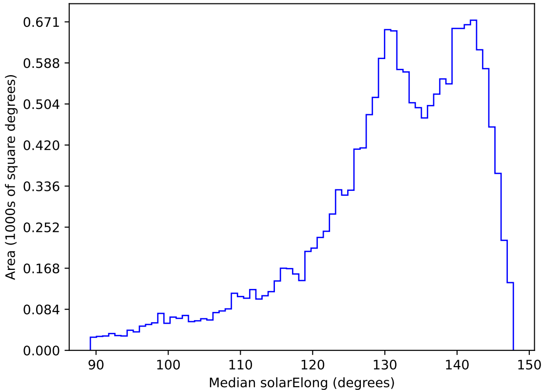
ddf_acor_sf25_lsf40_lsr10_v3.4_10yrs WFD r band: Median solarElong
