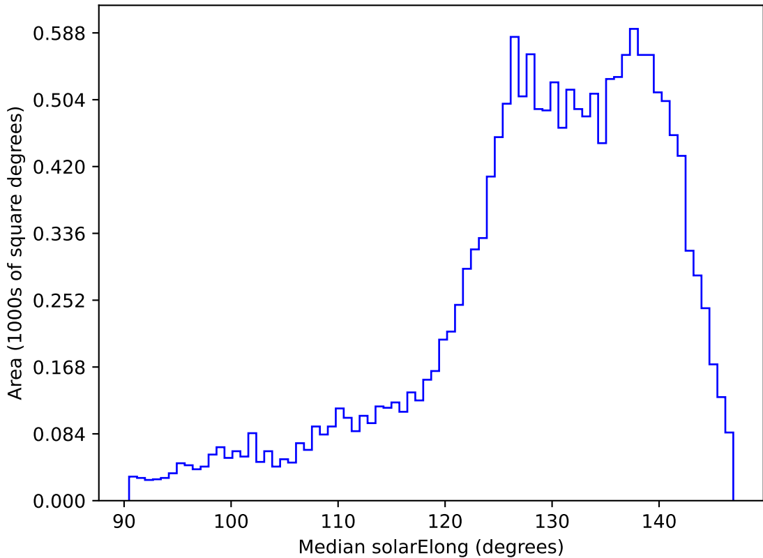
ddf_acor_sf25_lsf40_lsr10_v3.4_10yrs WFD i band: Median solarElong
