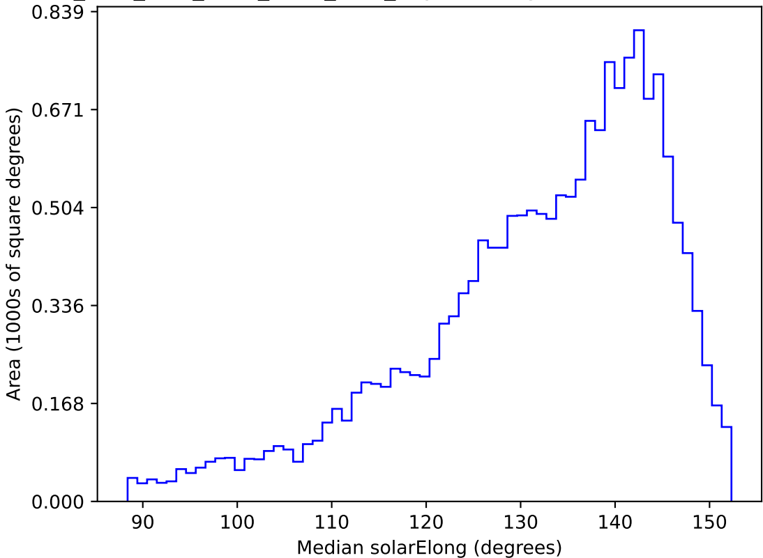
ddf_acor_sf25_lsf40_lsr10_v3.4_10yrs WFD g band: Median solarElong
