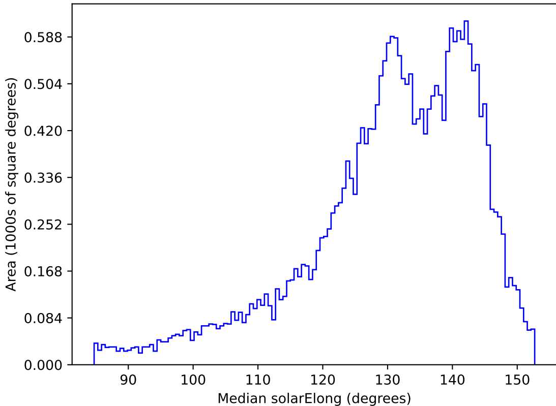
ddf_acor_sf25_lsf40_lsr10_v3.4_10yrs All sky r band: Median solarElong
